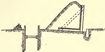
FIG. 11.—EXCAVATION-PLATFORM.
